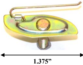
2619 UNIVERSAL MOULDING CLIP PLATE SIZE .500 X 1.375 10-24 X 3/4" BOLT $1.50
