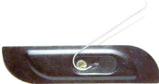
10794 UNIVERSAL MOULDING CLIP 10-24 X 3/4" BOLT PLATE LENGTH 4-7/16" $3.00
