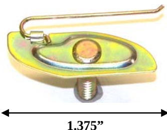
2619 UNIVERSAL MOULDING CLIP PLATE SIZE .500 X 1.375 10-24 X 3/4" BOLT $1.25
